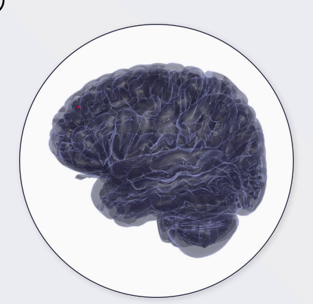
RUI-registered into Brain
